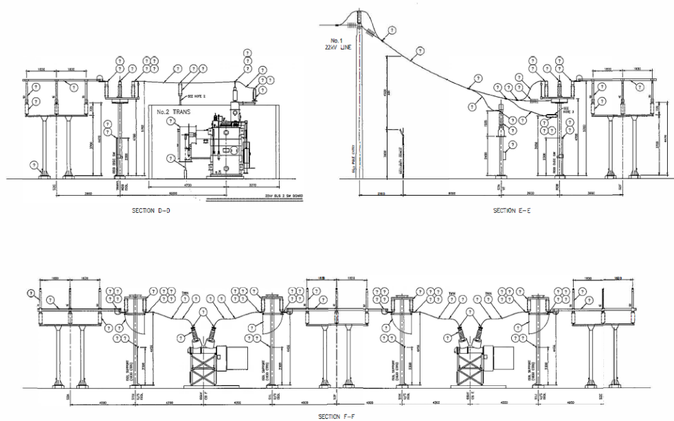
Figure 27 Typical substation infrastructure elevation
